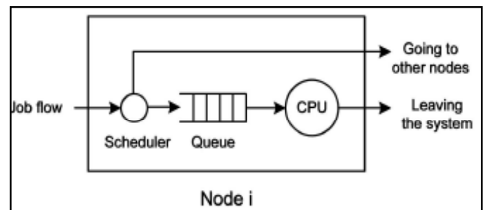
(b) Node Model of Rate Adjustment Policy
