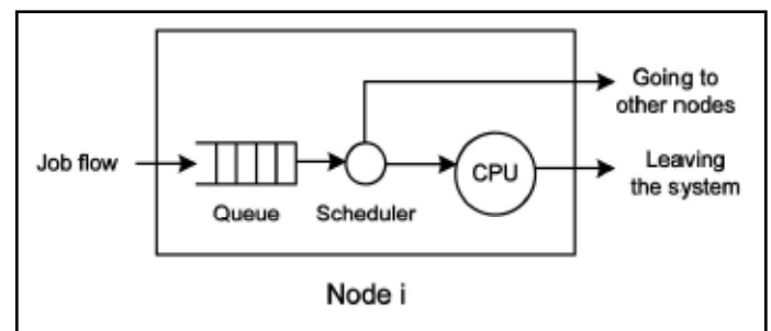
Fig. 2(a): Node Model of Queue Adjustment Policy
